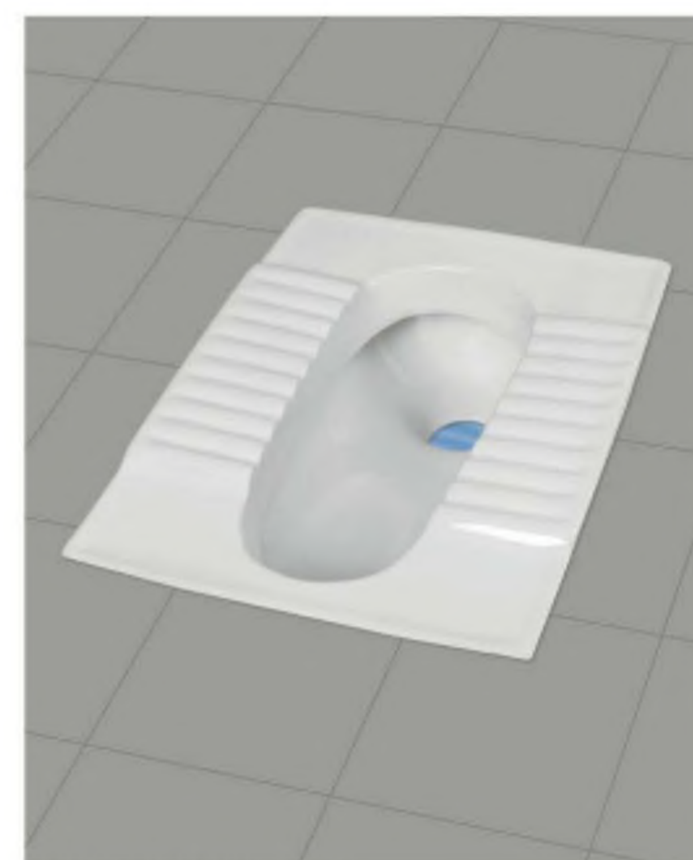
ORISSA PAN - 23" 610 x 455 x 250mm
